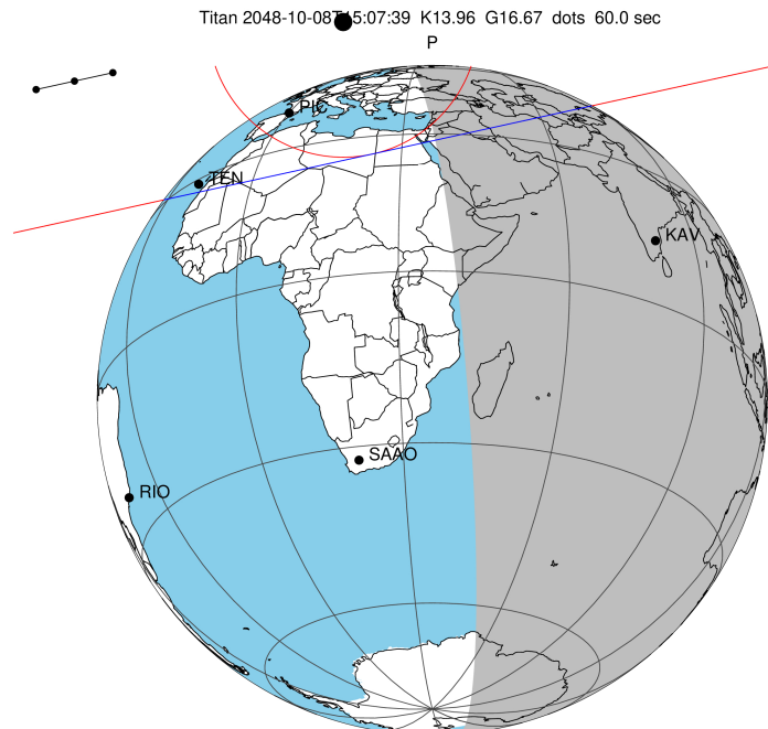
2048-10-08T15:07:39.5600 α: 18 39 49.7995 δ: -22 44 50.379 C/A 1.012" PA 347.59 deg v_sky +12.47 km/s D 10.09 AU Credit: Styled after SORA/Lucky Star
