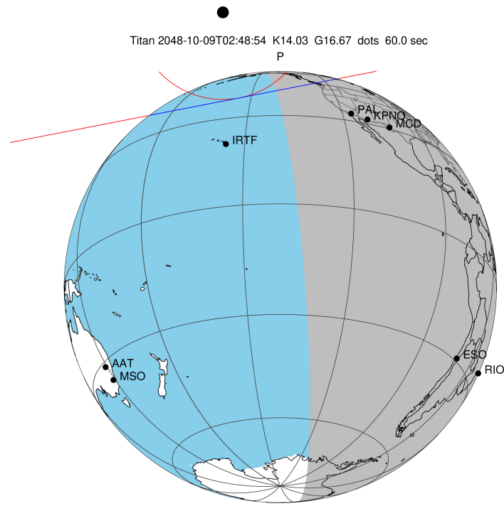
2048-10-09T02:48:54.7700 α: 18 39 55.1196 δ: -22 44 35.238 C/A 1.133" PA 348.96 deg v_sky +13.68 km/s D 10.10 AU Credit: Styled after SORA/Lucky Star
