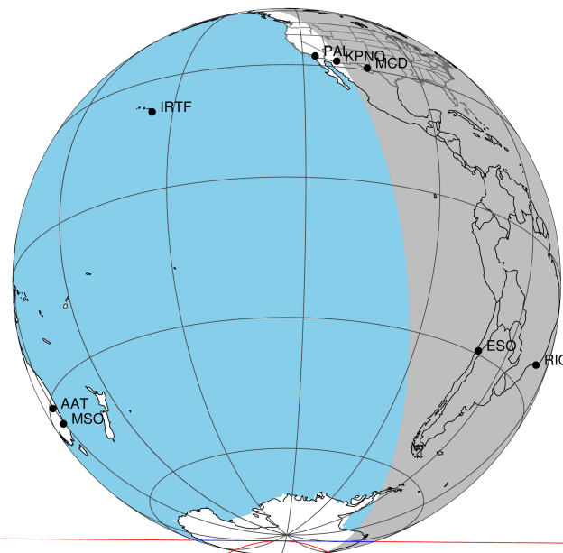
2048-10-30T00:28:15.3400 α: 18 45 25.8790 δ: -22 40 50.344 C/A 1.137" PA 180.44 deg v_sky +27.82 km/s D 10.43 AU Credit: Styled after SORA/Lucky Star
