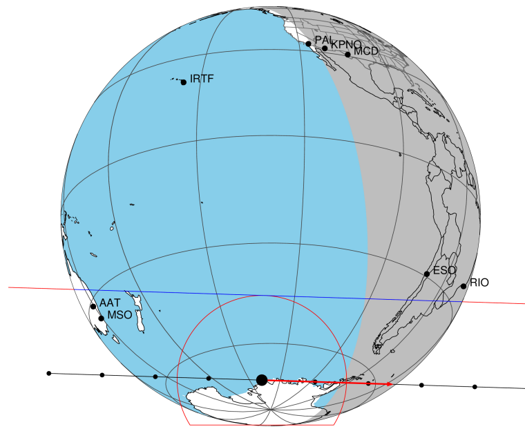
2048-10-31T00:45:50.0000 α: 18 45 48.7984 δ: -22 40 57.293 C/A 0.659" PA 181.83 deg v_sky +26.98 km/s D 10.45 AU Credit: Styled after SORA/Lucky Star
