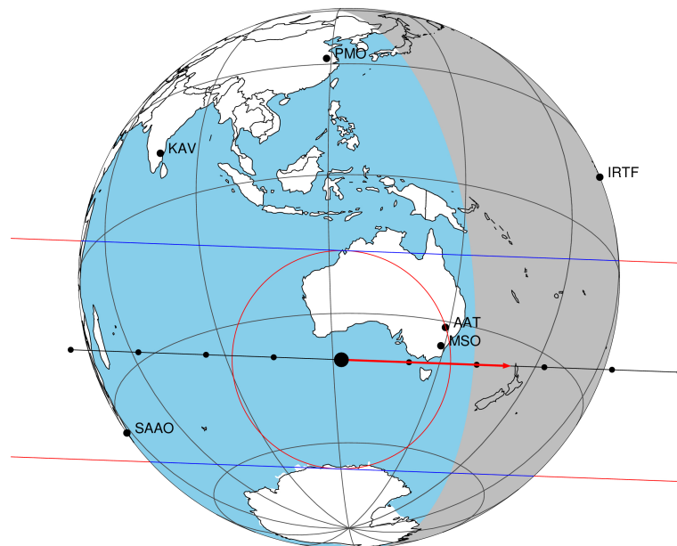
2048-10-31T07:49:49.9500 α: 18 45 55.2933 δ: -22 41 00.792 C/A 0.253" PA 182.14 deg v_sky +26.60 km/s D 10.45 AU Credit: Styled after SORA/Lucky Star
