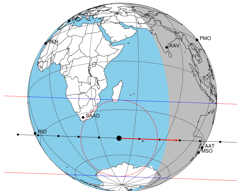
2048-11-02T12:39:24.2900 α: 18 46 40.0443 δ: -22 41 27.369 C/A 0.362" PA 182.07 deg v_sky +22.72 km/s D 10.48 AU
