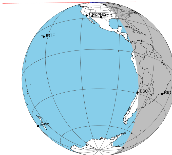
2048-11-03T22:58:27.2700 α: 18 47 05.3612 δ: -22 41 34.373 C/A 1.172" PA 359.34 deg v_sky +20.60 km/s D 10.49 AU Credit: Styled after SORA/Lucky Star
