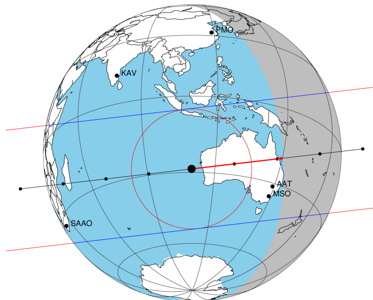
2048-11-11T08:07:19.1600 α: 18 49 25.8459 δ: -22 37 26.425 C/A 0.087" PA 173.28 deg v_sky +30.72 km/s D 10.60 AU Credit: Styled after SORA/Lucky Star
