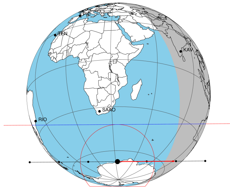
2048-11-15T12:52:52.9300 α: 18 51 18.9539 δ: -22 35 54.442 C/A 0.601" PA 179.59 deg v_sky +33.83 km/s D 10.66 AU Credit: Styled after SORA/Lucky Star
