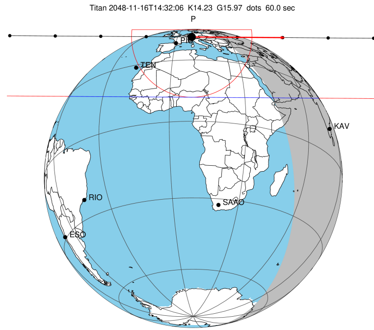
2048-11-16T14:32:06.6700 α: 18 51 47.5674 δ: -22 35 56.102 C/A 0.781" PA 0.42 deg v_sky +32.43 km/s D 10.67 AU Credit: Styled after SORA/Lucky Star
