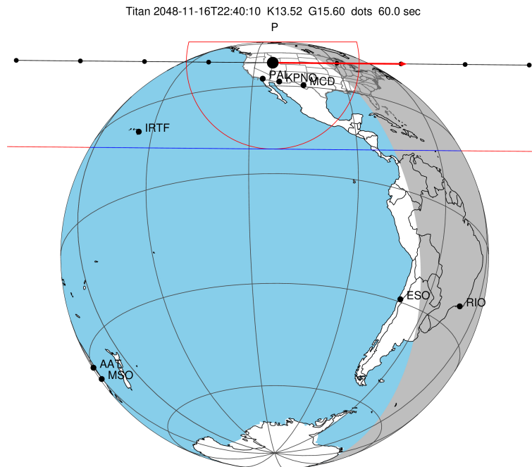
2048-11-16T22:40:10.6200 α: 18 51 56.3476 δ: -22 35 57.072 C/A 0.743" PA 0.54 deg v_sky +31.85 km/s D 10.67 AU Credit: Styled after SORA/Lucky Star
