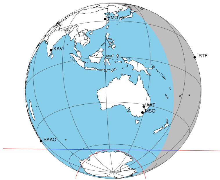
2048-11-17T06:46:36.6900 α: 18 52 04.9329 δ: -22 35 56.600 C/A 0.885" PA 180.57 deg v_sky +31.22 km/s D 10.68 AU Credit: Styled after SORA/Lucky Star
