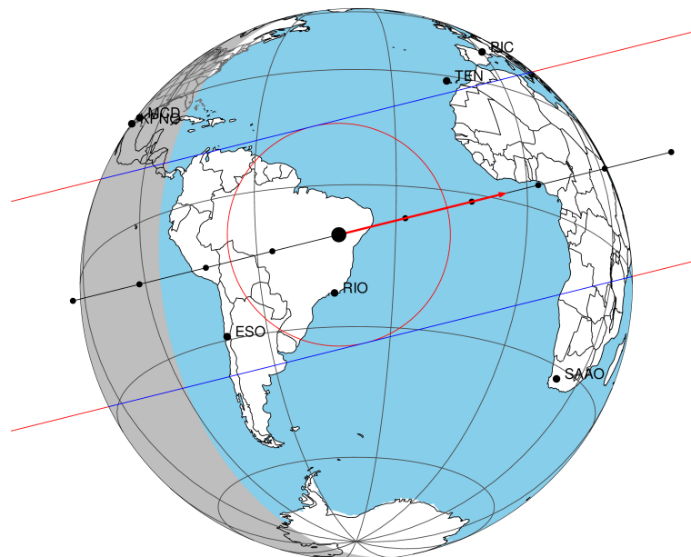
2049-02-27T11:45:09.5100 α: 19 40 02.0059 δ: -21 16 46.452 C/A 0.156" PA 346.04 deg v_sky +26.37 km/s D 10.68 AU Credit: Styled after SORA/Lucky Star
