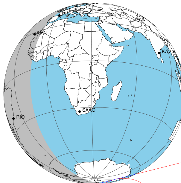
2049-02-28T07:00:57.8200 α: 19 40 18.6158 δ: -21 15 46.531 C/A 1.136" PA 165.76 deg v_sky +27.24 km/s D 10.67 AU Credit: Styled after SORA/Lucky Star
