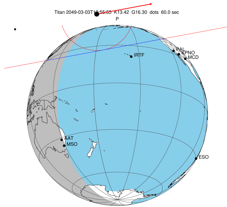
2049-03-03T19:55:55.5200 α: 19 41 41.0913 δ: -21 11 26.092 C/A 0.946" PA 349.43 deg v_sky +32.52 km/s D 10.64 AU Credit: Styled after SORA/Lucky Star
