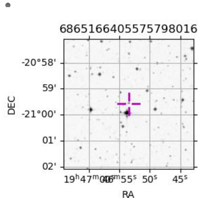
2049-03-18T22:28:01.2000 α: 19 46 53.5276 δ: -20 59 34.766 C/A 1.129" PA 167.06 deg v_sky +24.96 km/s D 10.43 AU Credit: Styled after SORA/Lucky Star
