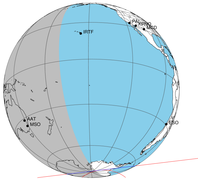
2049-03-27T17:22:24.0800 α: 19 49 43.9066 δ: -20 55 05.247 C/A 1.131" PA 173.12 deg v_sky +15.59 km/s D 10.29 AU
