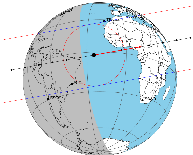
2049-04-05T08:19:03.9800 α: 19 51 28.2459 δ: -20 48 33.563 C/A 0.279" PA 349.82 deg v_sky +19.34 km/s D 10.16 AU Credit: Styled after SORA/Lucky Star
