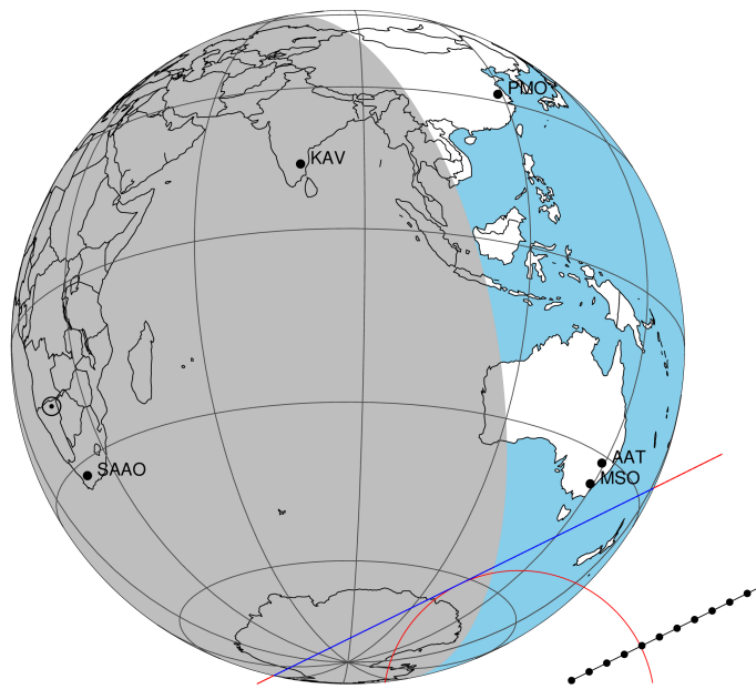
2049-05-13T22:40:43.8200 α: 19 54 53.0705 δ: -20 44 35.501 C/A 1.091" PA 153.73 deg v_sky - 6.20 km/s D 09.52 AU Credit: Styled after SORA/Lucky Star
