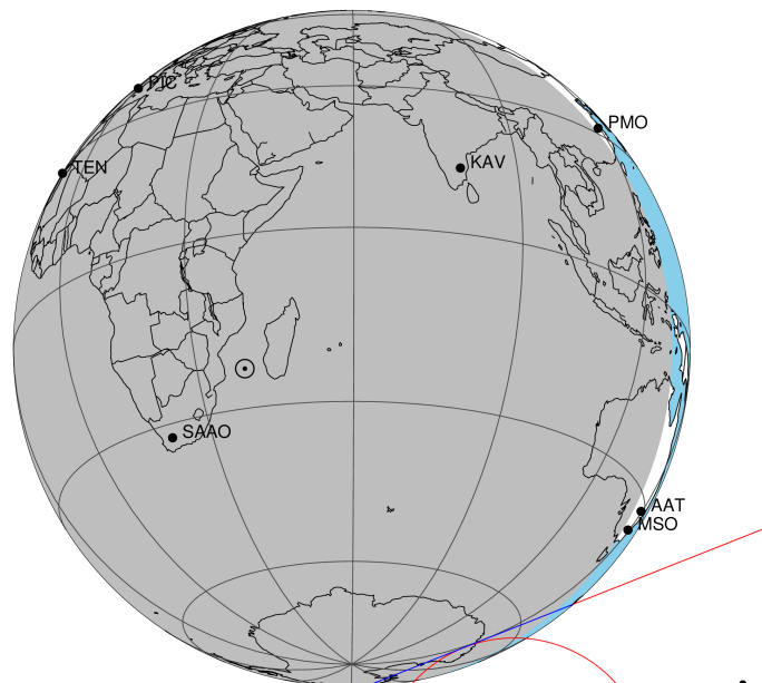
2049-06-27T21:25:10.0800 α: 19 46 38.1557 δ: -21 08 39.608 C/A 1.310" PA 158.39 deg v_sky -15.45 km/s D 09.04 AU
