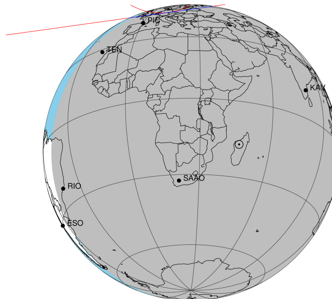
2049-08-03T21:01:15.6600 cc: 19 35 16.8954 & -21 40 46.336 C/A 1.326" PA 352.06 deg v_sky -23.79 km/s D 09.03 AU
