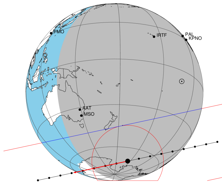
2049-09-03T08:54:43.800000 cc: 19 28 34.6931 d: -21 58 00.170 C/A 0.749" PA 167.90 deg v_sky -13.74 km/s D 09.32 AU Credit: Styled after SORA/Lucky Star
