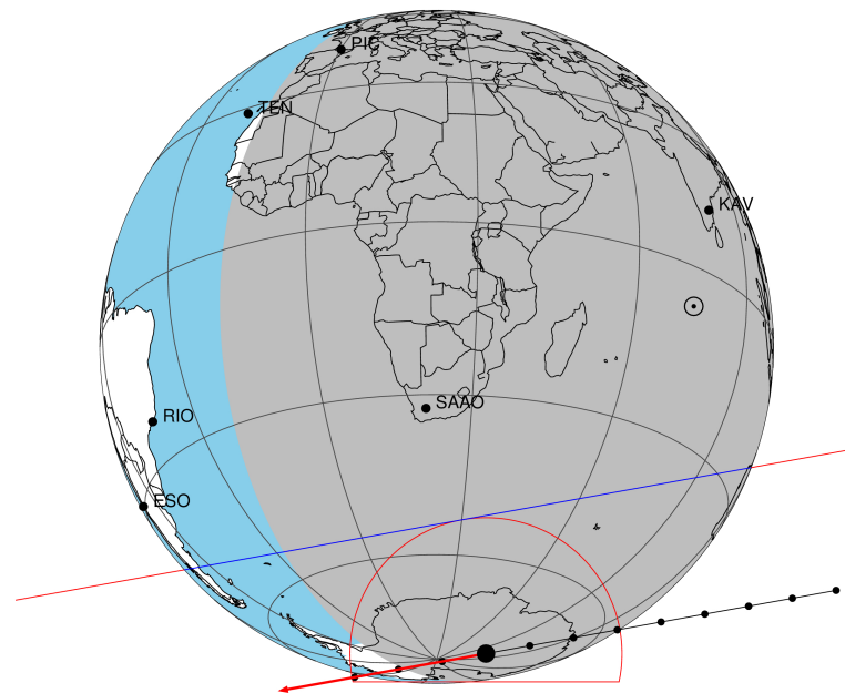
2049-09-03T19:06:04.50000 cc: 19 28 29.37474 & -21 58 14.63315 C/A 0.870" PA 169.78 deg v_sky -14.04 km/s D 09.32 AU Credit: Styled after SORA/Lucky Star
