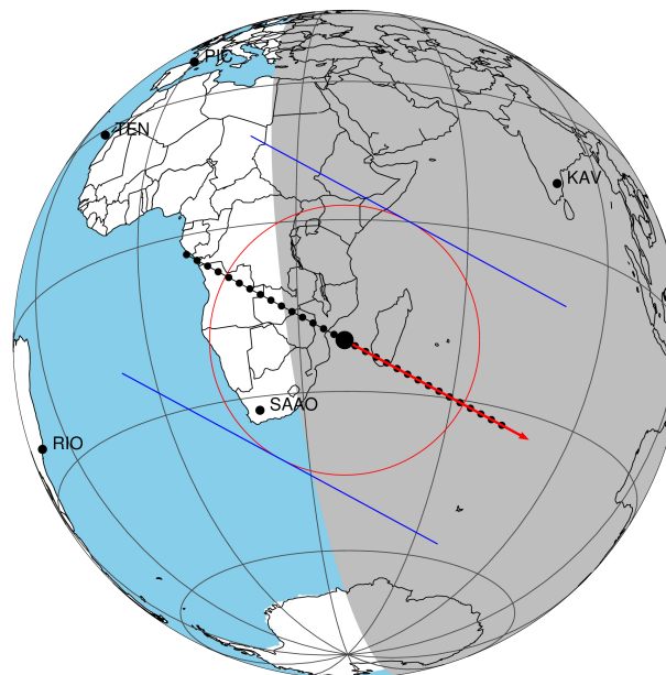
2049-10-03T16:03:29.0900 α: 19 27 24.1887 δ: -22 02 16.902 C/A 0.006" PA 28.32 deg v_sky + 3.80 km/s D 09.77 AU Credit: Styled after SORA/Lucky Star
