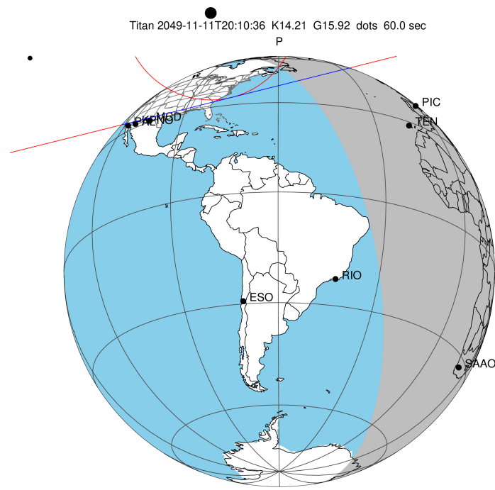
2049-11-11T20:10:36.5000 α: 19 34 40.9764 δ: -21 47 39.746 C/A 1.050" PA 345.97 deg v_sky +22.98 km/s D 10.40 AU Credit: Styled after SORA/Lucky Star
