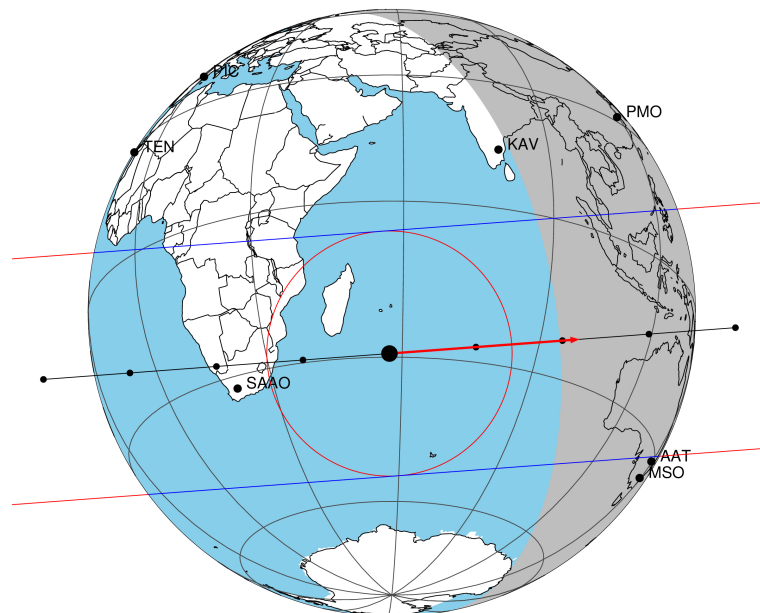
2049-11-17T12:00:41.4000 α: 19 36 49.93556 δ: -21 43 05.313 C/A 0.112" PA 175.74 deg v_sky +30.35 km/s D 10.49 AU
