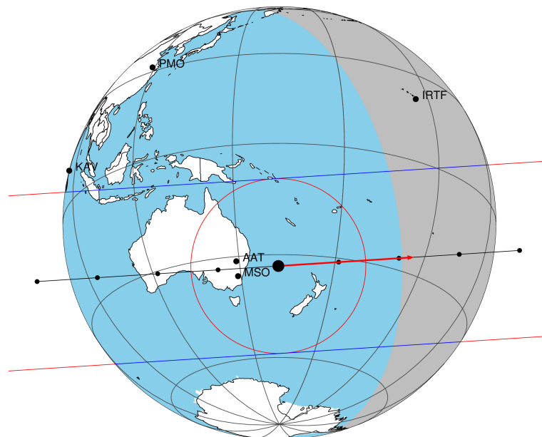
2049-11-18T04:59:03.2300 α: 19 37 07.1908 δ: -21 42 48.597 C/A 0.166" PA 176.28 deg v_sky +29.65 km/s D 10.50 AU Credit: Styled after SORA/Lucky Star
