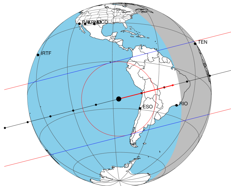
2049-11-26T21:00:16.1700 α: 19 40 00.5441 δ: -21 36 41.800 C/A 0.034" PA 165.60 deg v_sky +27.13 km/s D 10.61 AU Credit: Styled after SORA/Lucky Star
