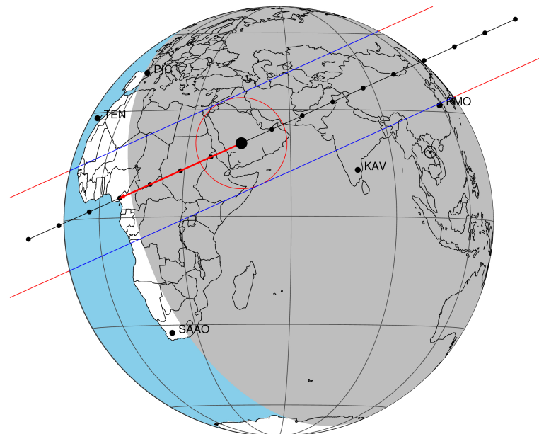
2025-11-12T16:45:45.8500 α: 23 59 18.6100 δ: -01 33 51.532 C/A 0.121" PA 335.68 deg v_sky -16.52 km/s D 29.25 AU
