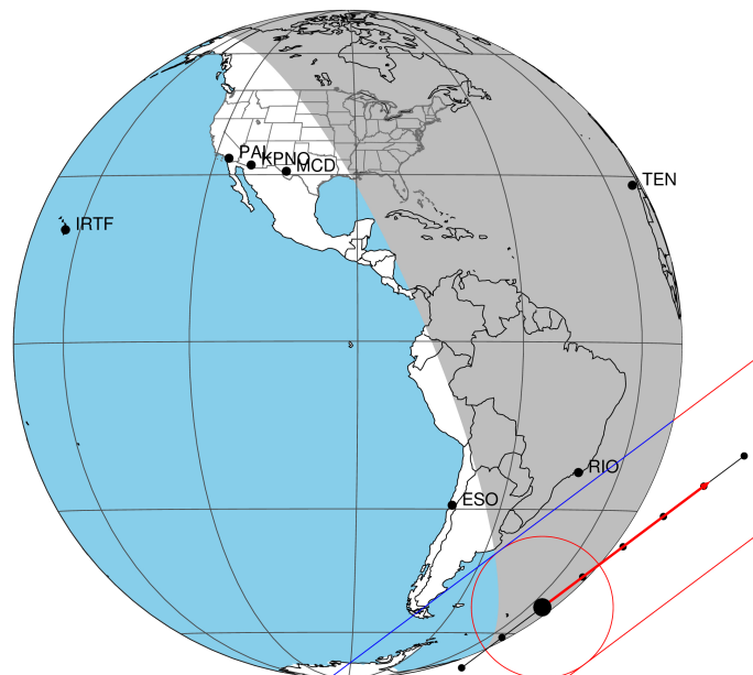
2027-01-05T23:14:15.2700 α: 00 07 19.0514 δ: -00 42 13.104 C/A 0.286" PA 143.12 deg v_sky +16.04 km/s D 30.09 AU Credit: Styled after SORA/Lucky Star
