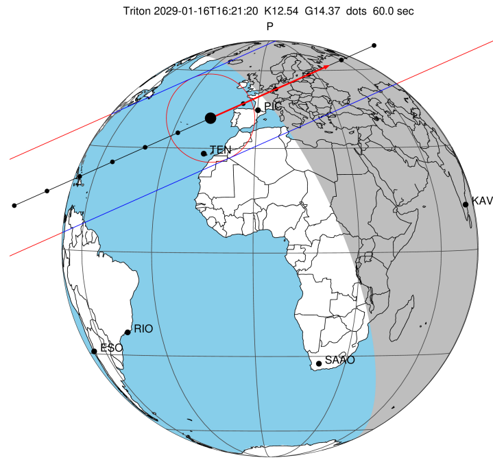
2029-01-16T16:21:20.6000 α: 00 24 10.2730 δ: +01 02 14.470 C/A 0.201" PA 335.99 deg v_sky +18.27 km/s D 30.19 AU Credit: Styled after SORA/Lucky Star
