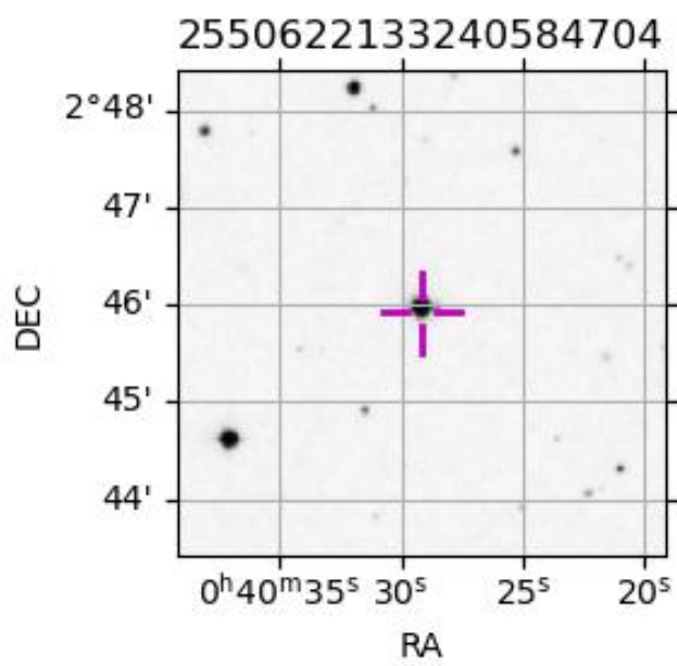
2029-06-08T11:30:48.1400 α: 00 40 29.1667 δ: +02 45 54.805 C/A 0.270" PA 352.41 deg v_sky +14.45 km/s D 30.24 AU Credit: Styled after SORA/Lucky Star
