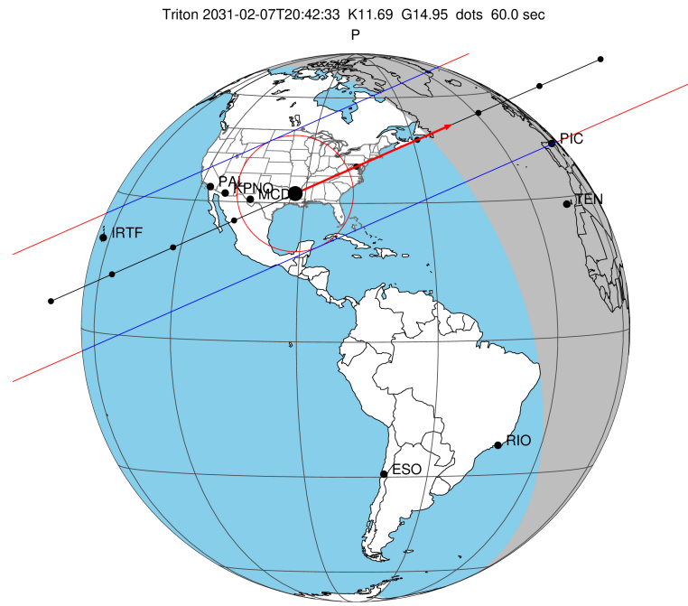
2031-02-07T20:42:33.7100 α: 00 42 01.5793 δ: +02 52 55.875 C/A 0.155" PA 336.22 deg v_sky +25.86 km/s D 30.44 AU Credit: Styled after SORA/Lucky Star
