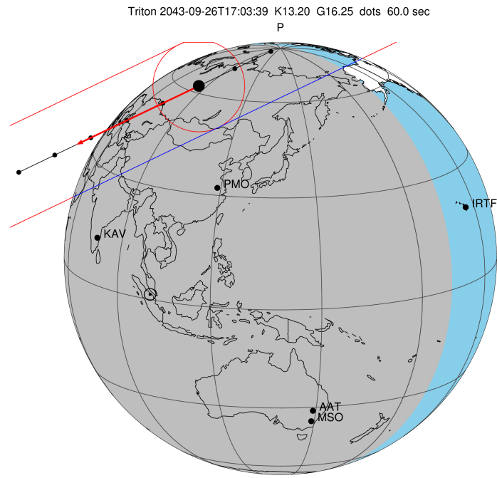
2043-09-26T17:03:39.5400 α: 02 38 45.3332 δ: +13 34 09.933 C/A 0.267" PA 334.37 deg v_sky -19.63 km/s D 29.02 AU Credit: Styled after SORA/Lucky Star
