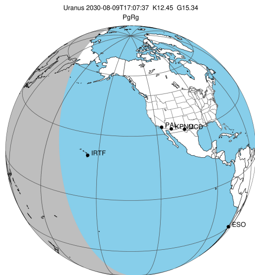
2030-08-09T17:07:37.5200 ex: 05 22 43.1633 s: +23 13 38.877 C/A 0.902° PA 176.01 deg v_sky +23.28 km/s D 19.74 AU Credit: Styled after SORA/Lucky Star
