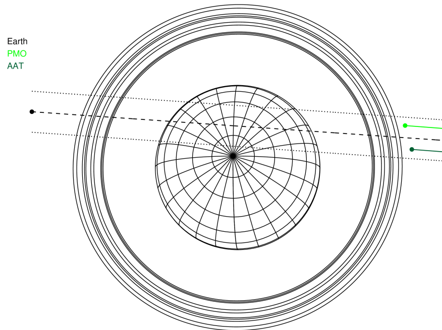
Uranus 2030-08-09T17:07:37 K12.45 G15.34 PgRg
