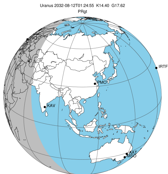
2032-08-12T01:24:55.2300 ex: 05 59 39.8600 s: +23 36 54.227 C/A 2.039° PA 179.61 deg v_sky +25.69 km/s D 19.69 AU Credit: Styled after SORA/Lucky Star
