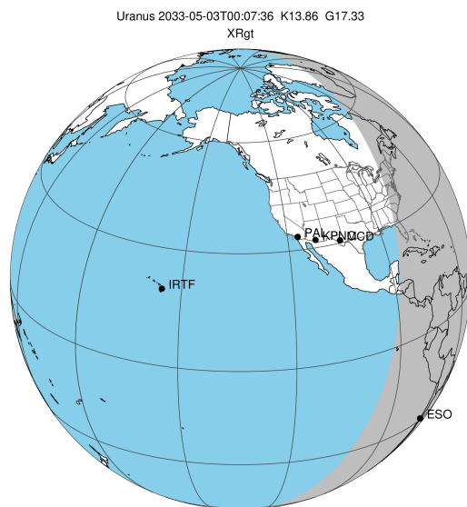
2033-05-03T00:07:36.4600 ex: 05 53 41.7317 s: +23 38 46.937 C/A 2.768° PA 179.36 deg v_sky +27.02 km/s D 19.68 AU Credit: Styled after SORA/Lucky Star
