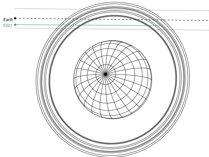
Uranus 2033-05-03T00:07:36 K13.86 G17.33 XRgt
