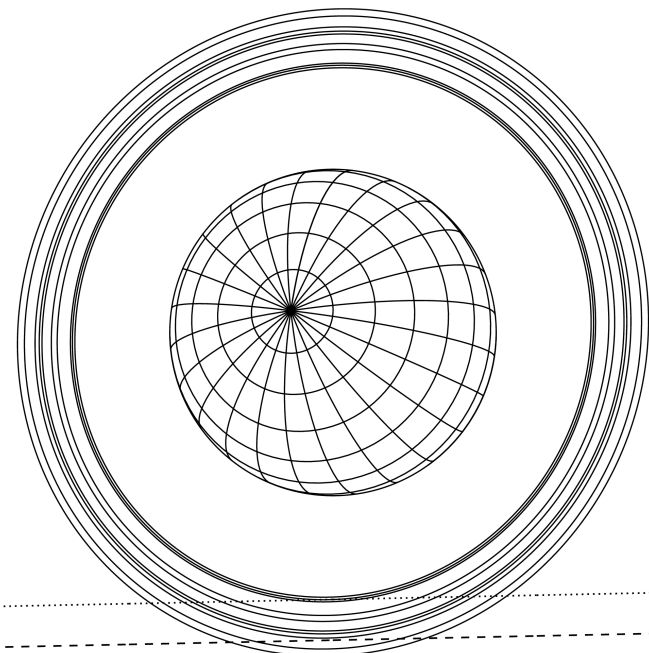
Uranus 2034-04-28T17:54:34 K14.21 G17.33 XRg
