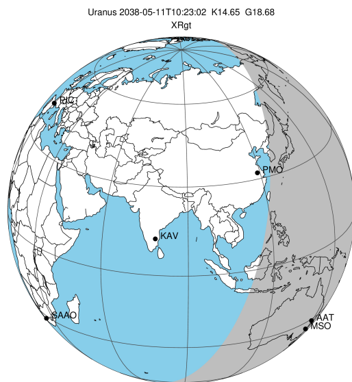
2038-05-11T10:23:02.7800 ex: 07 28 34.9637 s: +22 21 33.629 C/A 3.279° PA 188.99 deg v_sky +21.35 km/s D 19.17 AU Credit: Styled after SORA/Lucky Star
