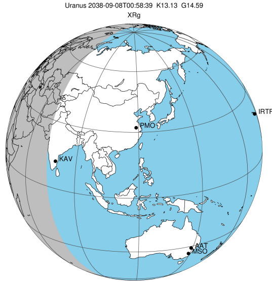
2038-09-08T00:58:39.500000 ex: 07 56 03.6839 8: +21 15 30.216 C/A 2.265° PA 190.56 deg v_sky +26.41 km/s D 19.32 AU Credit: Styled after SORA/Lucky Star
