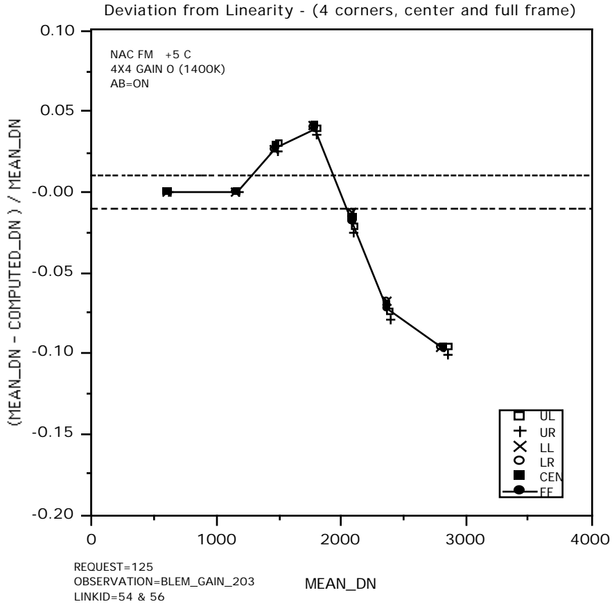
Figure 2.3-1 - NAC FM 4x4 Linearity Breakdown
